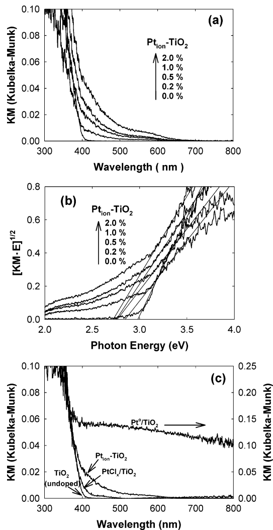
Figure 1. (a) Diffuse reflectance UV/vis spectra of \text{Pt}_{\text{ion}}\text{-TiO}_2 as a function of the Pt content. (b) Plot of the modified Kubelka–Munk (KM) function versus photon energy ( E ) for the reflectance spectra of \text{Pt}_{\text{ion}}\text{-TiO}_2 samples. (c) Comparison of the diffuse reflectance spectra of \text{Pt}_{\text{ion}}\text{-TiO}_2 with \text{Pt}^0/\text{TiO}_2 and \text{PtCl}_x/\text{TiO}_2 .
