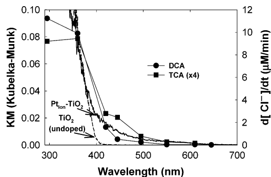
Figure 11. Wavelength-dependent PCDs (chloride production) of DCA (under air equilibration) and TCA (under N 2 saturation) compared with the diffuse reflectance spectra of Pt ion -TiO 2 (0.5 atom %).
