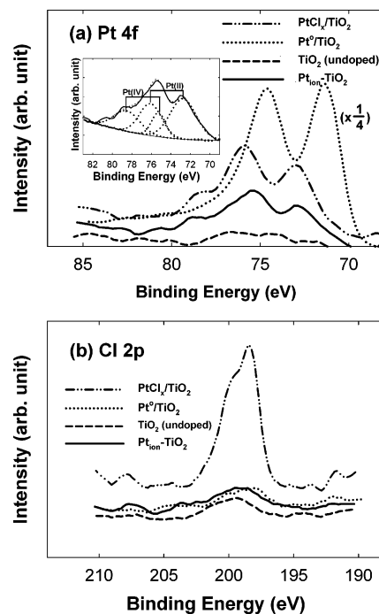
Figure 2. XPS spectra of various Pt-modified \text{TiO}_2 samples in the (a) Pt 4f and (b) Cl 2p band region. The Pt content in all samples was the same at 0.5 atom %.
