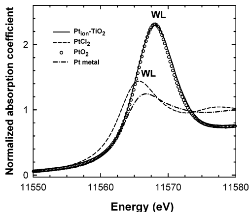
Figure 3. Pt L_{\text{III}} edge XANES spectrum for the \text{Pt}_{\text{ion}}\text{-TiO}_2 compound (solid lines), in comparison with those for the references \text{PtO}_2 (circles), \text{PtCl}_2 (dashed lines), and Pt metal (dot–dashed lines).
