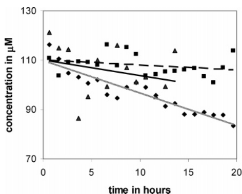
Figure 6. Concentration of 15 N-carboplatin (original concentration, 110 μM) as a function of time derived from HSQC NMR intensities, with linear fits to the data. Carboplatin in water at initial pH 7.5 is squares and dashed line; carboplatin in 10 mM carbonate buffer at pH 8.6 is triangles and solid line; and carboplatin in 23.8 mM carbonate buffer at pH 8.6 is diamonds and gray line.
